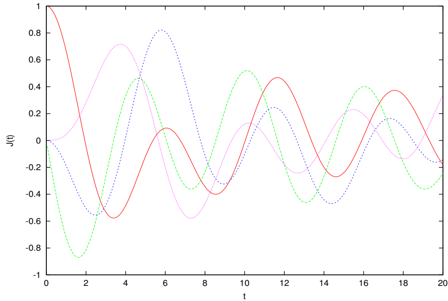
FIG. 1.1. F-B. functions i^n \mathcal{J}_n(\mu; t) , n = 0, 1, 2, 3 , for a Julia set measure with \lambda = 2.9 . Different curves can be distinguished from the behavior at the origin: \mathcal{J}_n(\mu; t) \sim t^n , as in the Bessel case.
