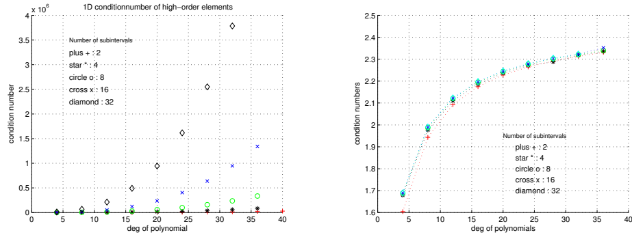
FIG. 6.2. Condition numbers of \tilde{L}_N (left) and \widehat{B}_h^{-1} \tilde{L}_N (right).
