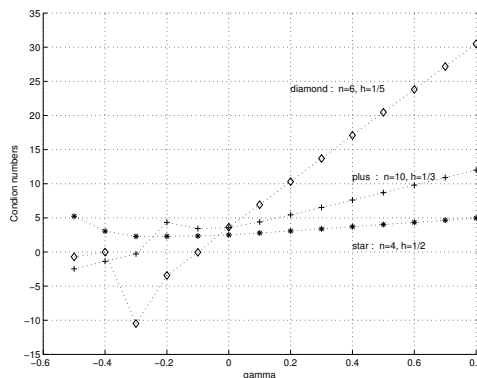
FIG. 6.1. Condition numbers of \widehat{B}_h^{-1} \widetilde{L}_N according to \gamma
