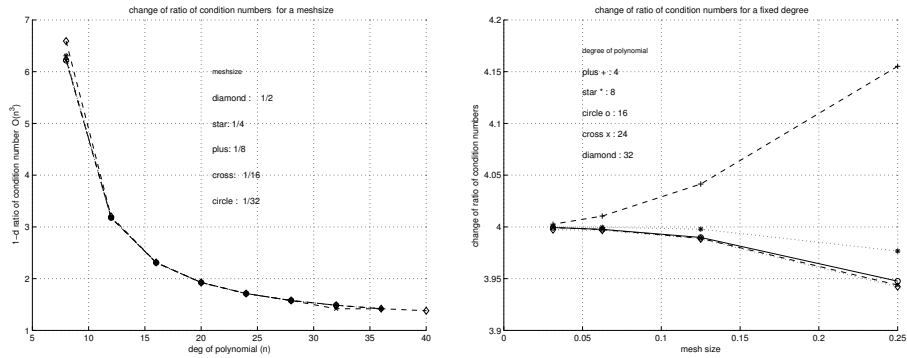
FIG. 6.3. Increasing rates of condition numbers of \tilde{L}_N .
