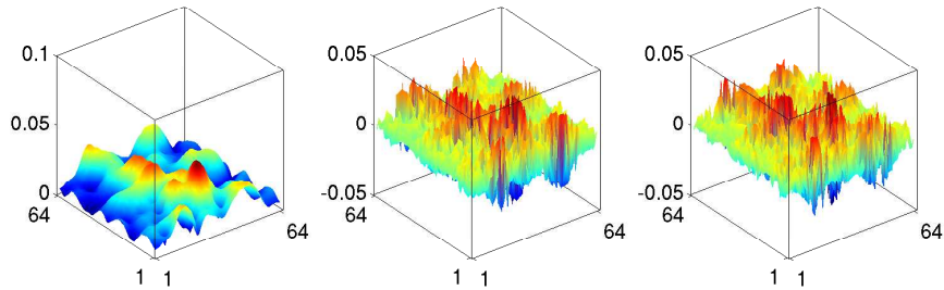
FIG. 2.3. Modulus, real and imaginary part of an algebraically smooth error after 50 Gauss-Seidel iterations for \beta = 5 on a 64 \times 64 grid, no odd-even reduction.
