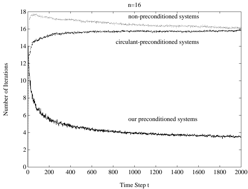
FIG. 4. Numbers of Iterations for Convergence at Each Time Step with n = 16 .
