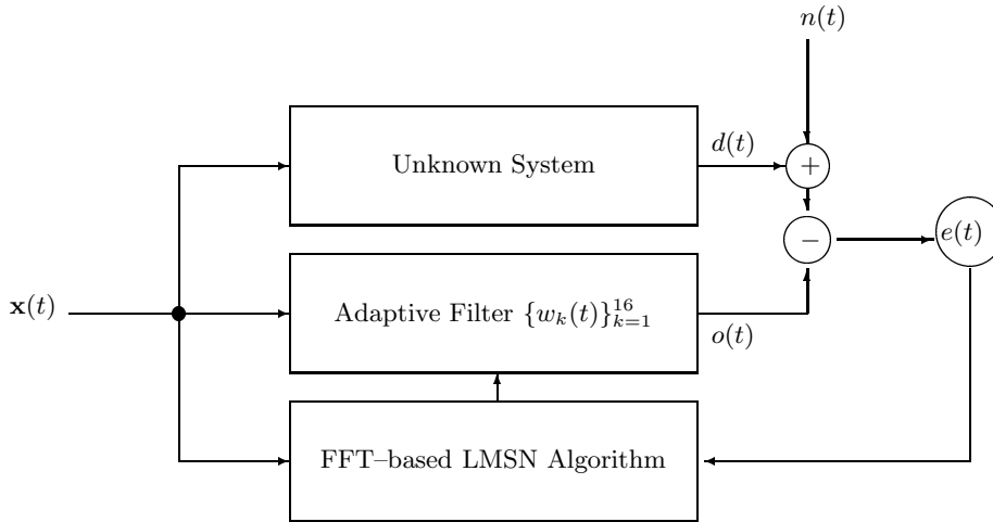
FIG. 2. Adaptive Filtering Simulation Model
