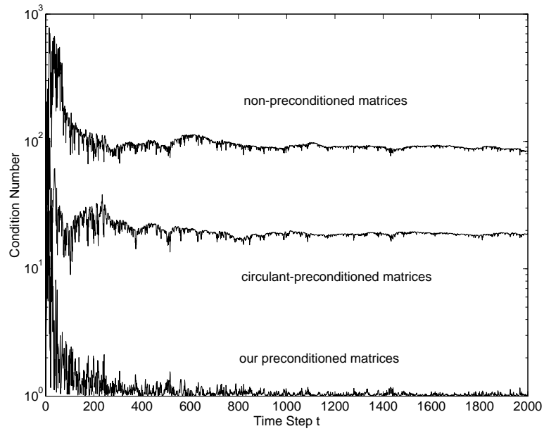
FIG. 3. Condition Numbers of Different Preconditioned Matrices.
