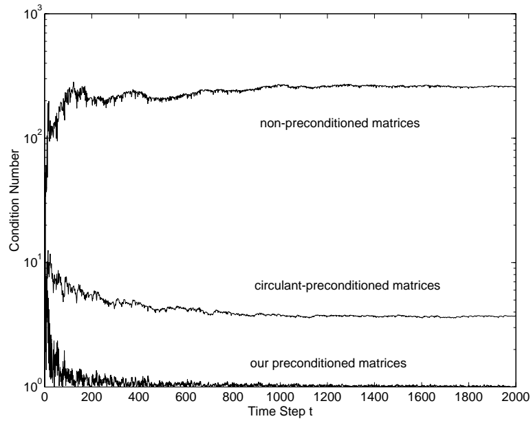
FIG. 9. Condition Numbers of Different Preconditioned Matrices.
