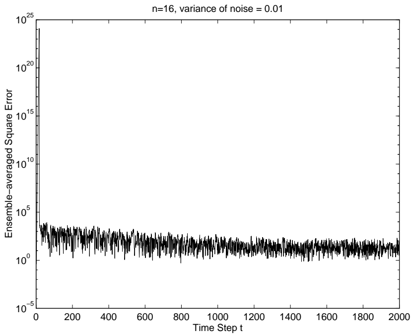
FIG. 12. Learning Curves of the Fast Transversal Filter Algorithms.
