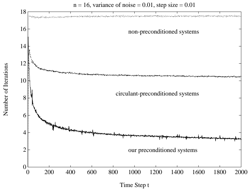
FIG. 10. Numbers of Iterations for Convergence at Each Time Step with n = 16 .
