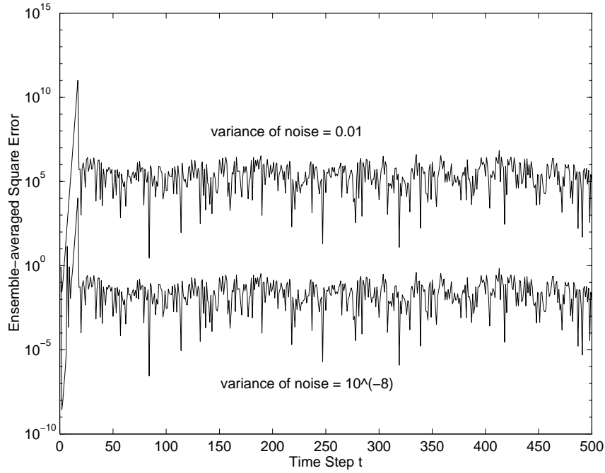
FIG. 7. Learning Curves of the Fast Transversal Filter Algorithms.
