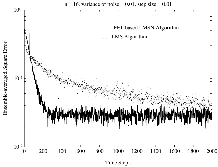
FIG. 11. Learning Curves of the FFT-based LMSN and LMS Algorithms.
