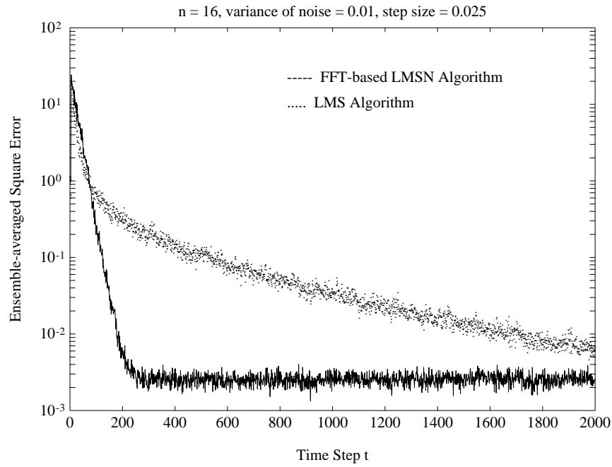
FIG. 5. Learning Curves of the FFT-based LMSN and LMS Algorithms.
