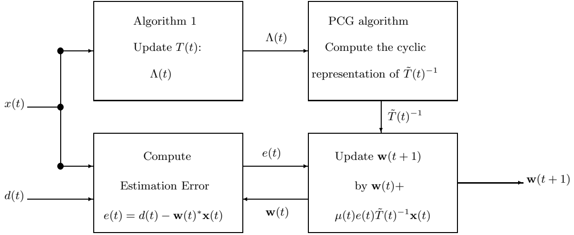
FIG. 1. Block Diagram of the FFT-based LMSN Algorithm.
