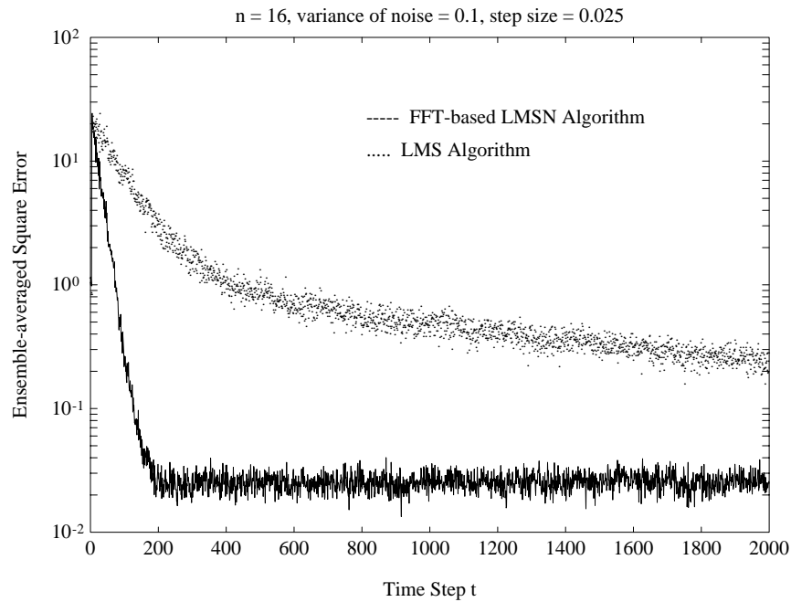
FIG. 6. Learning Curves of the FFT-based LMSN and LMS Algorithms.
