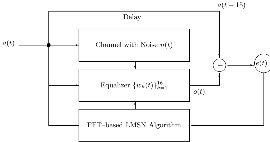
FIG. 8. The Equalization Problem used for Simulation.
